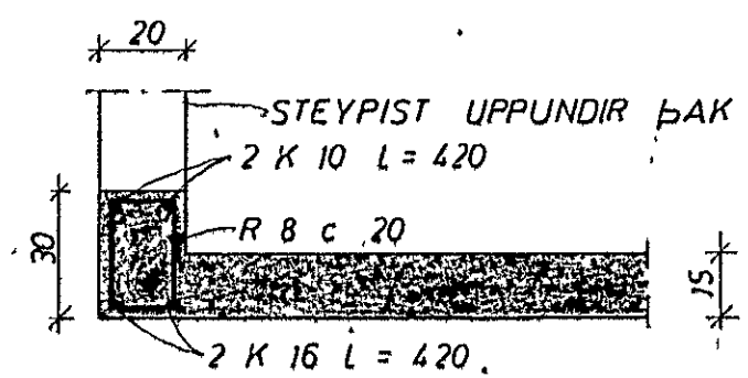
SNID C 1:20
