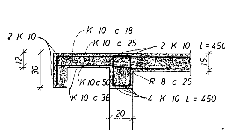
SNID A 1:20
