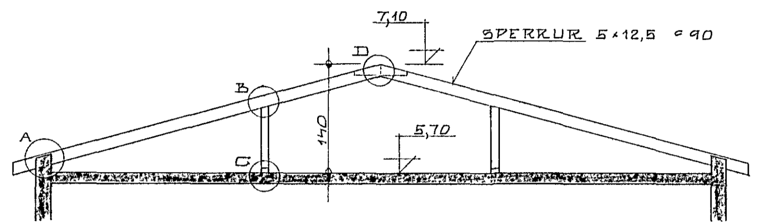
SNIED 11 - 11 1 50
