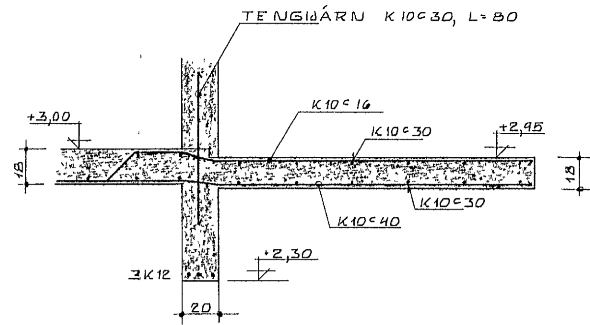
SNID 7-7 1:20
