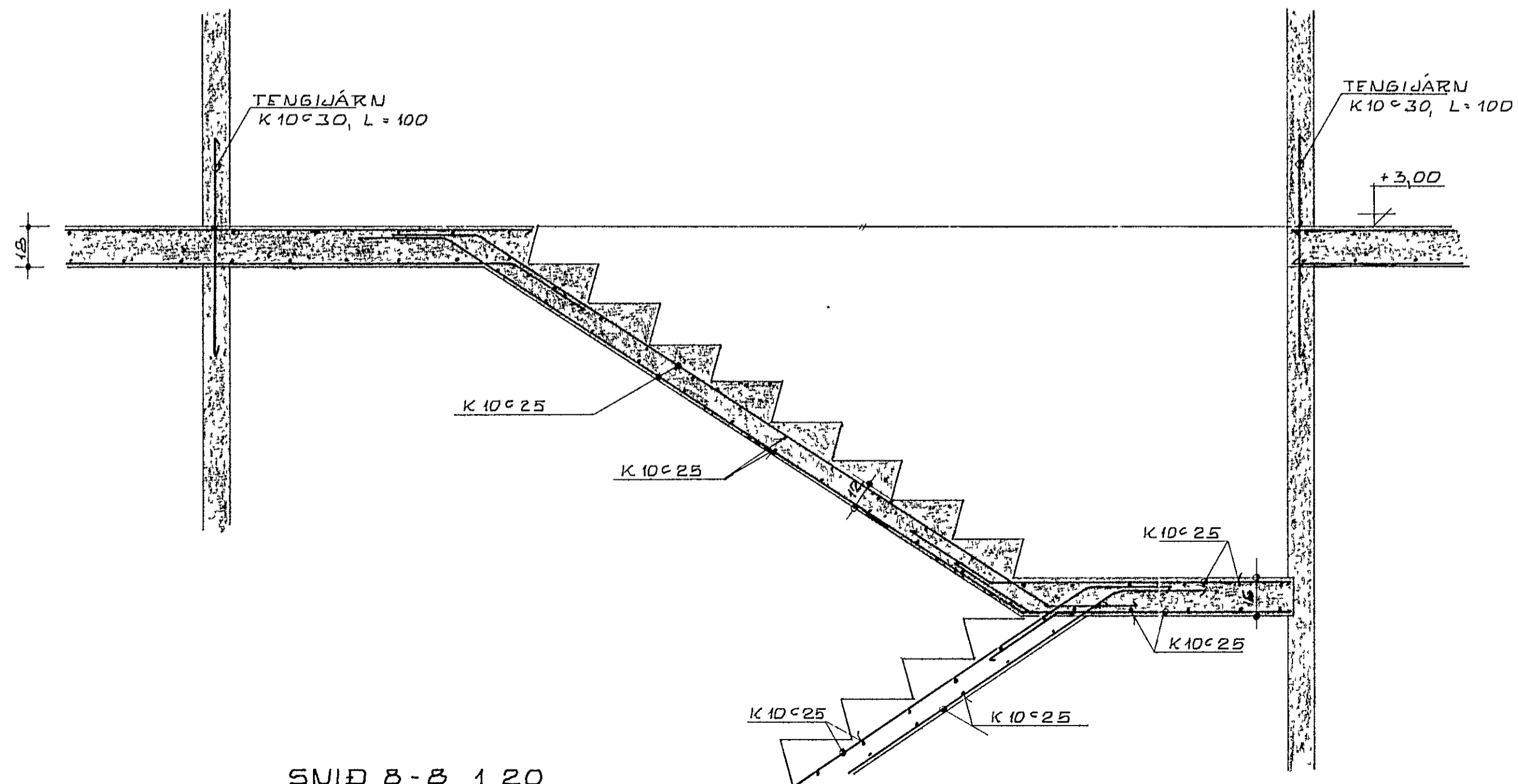
SNID 8-8 1:20
