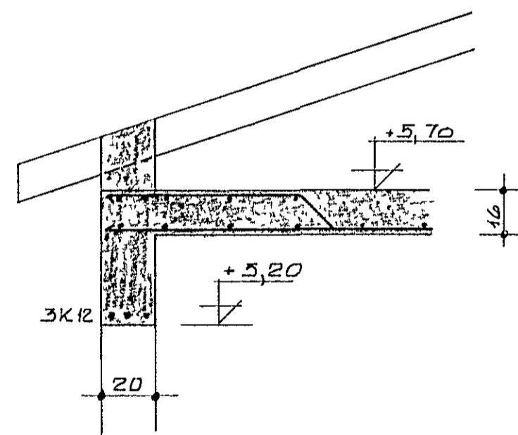
SNID 9-9 1:20
