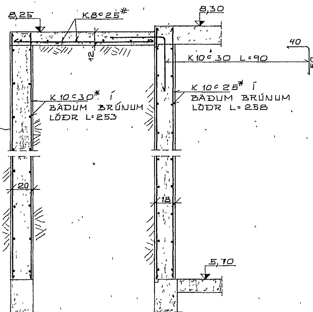
SNID 8-8 1:20
