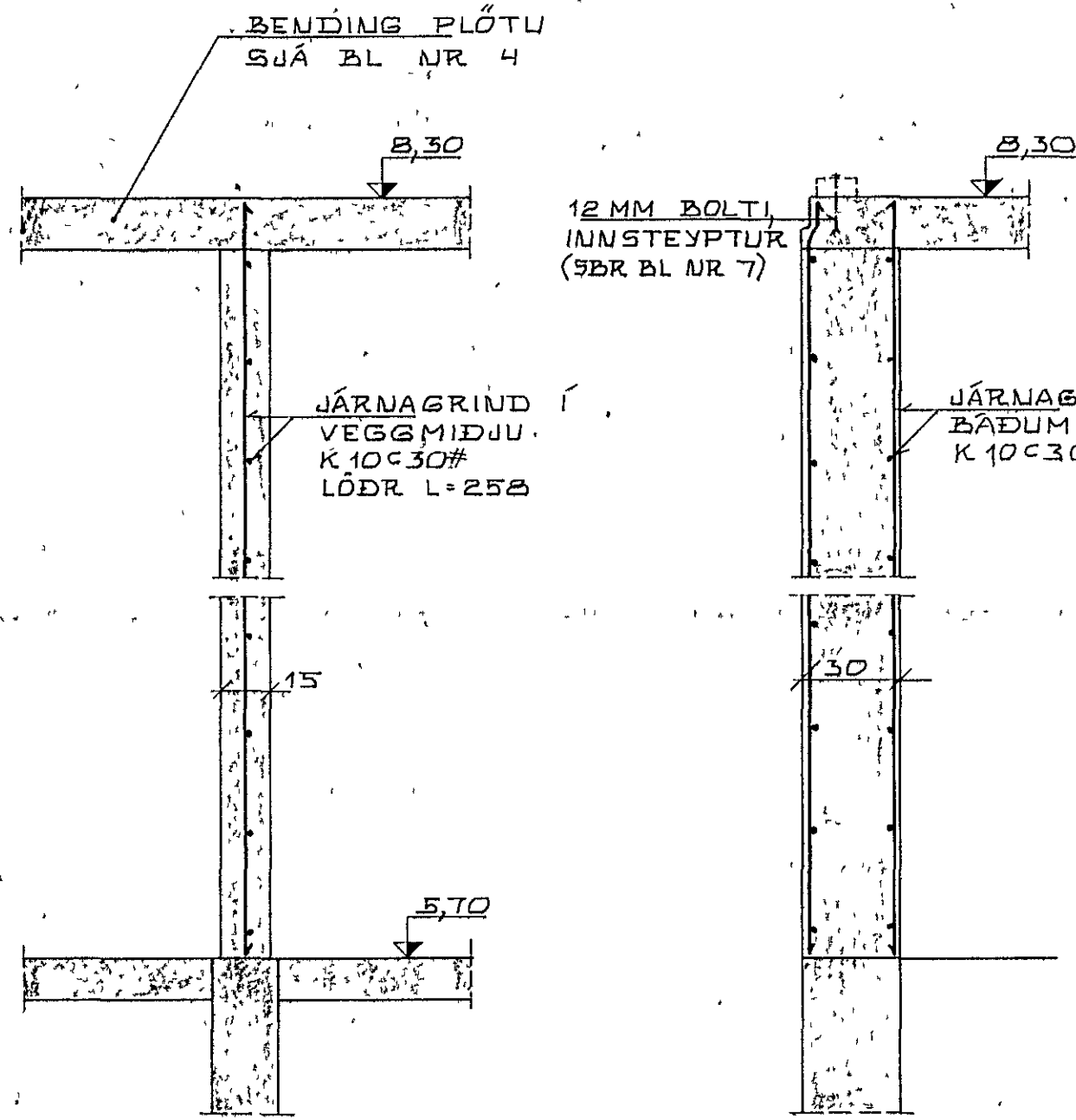
SNID 3-3 1:20
