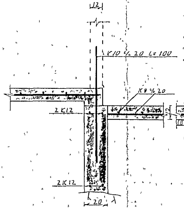
SNID C-C 1:20
