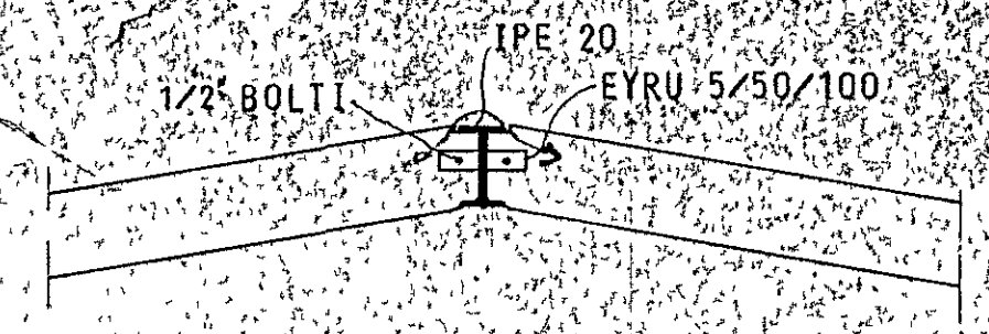
SNID B 1:20
