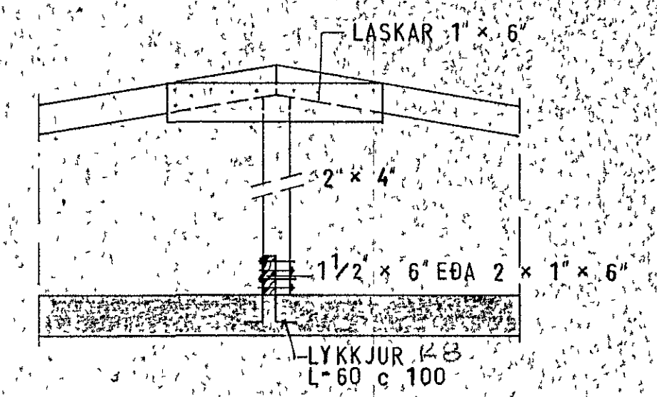
SNID C 1:20
