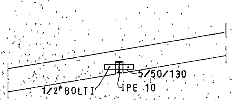
SNID F 1:20
