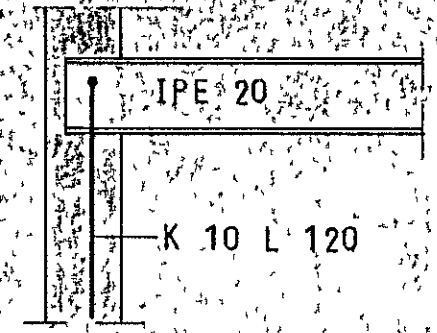
SNID A 1:20
