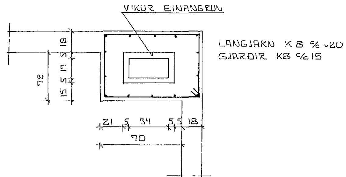
SNID C-C 1:20
