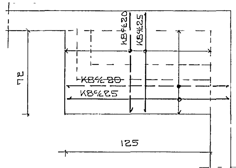
SNID A-A 1:20 BENDING NEÐRI HILLU
