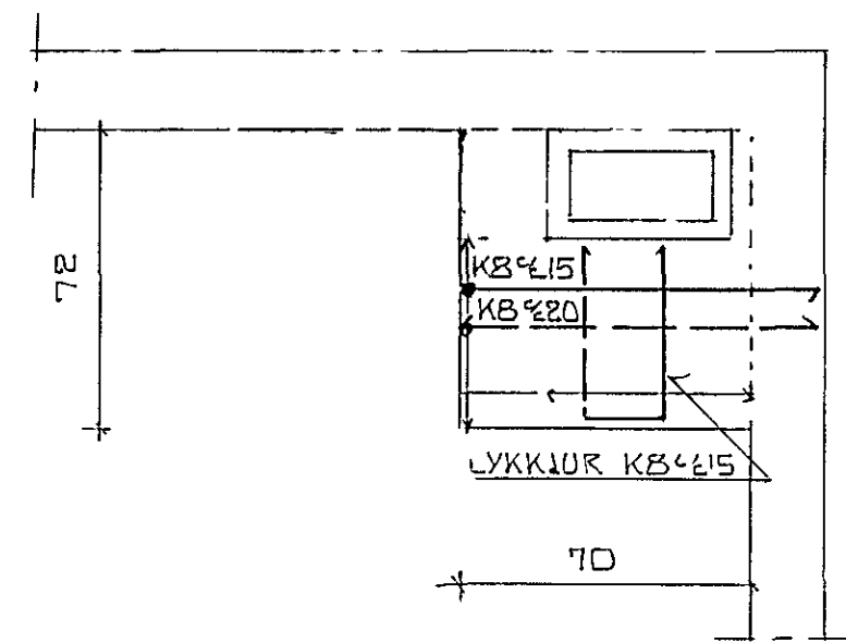
SNID B-B 1:20 BENDING EFRI HILLU
