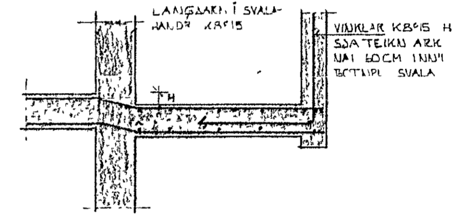
SNID C-C 1:20
