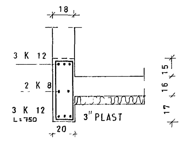
SNID A 1:20
