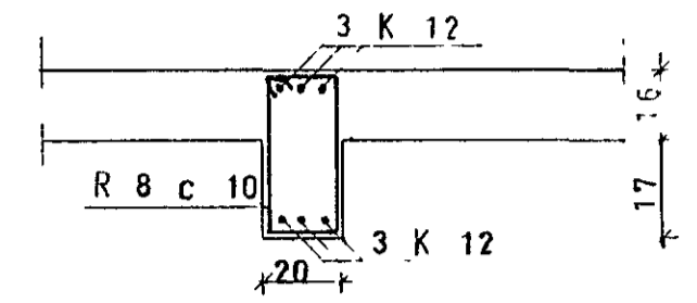
SNID B 1:20
