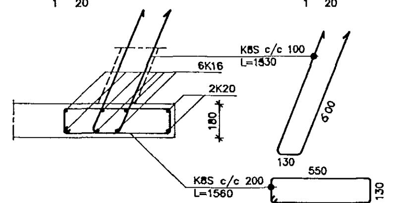
S2-06 1 20
