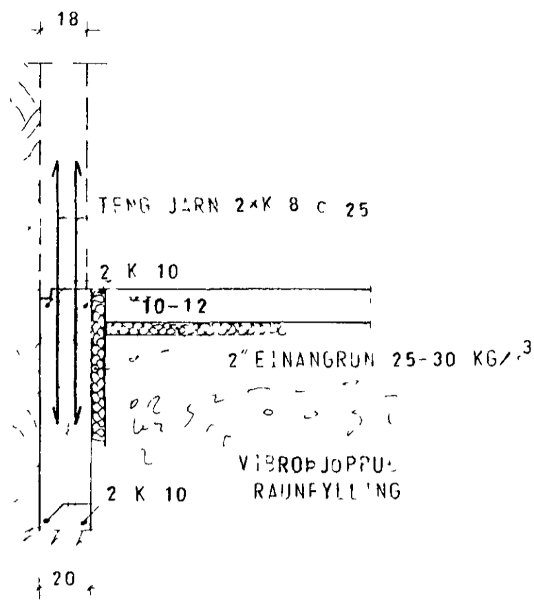
SNID A 1:20
