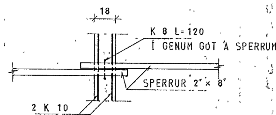
SNID C, 1:20
