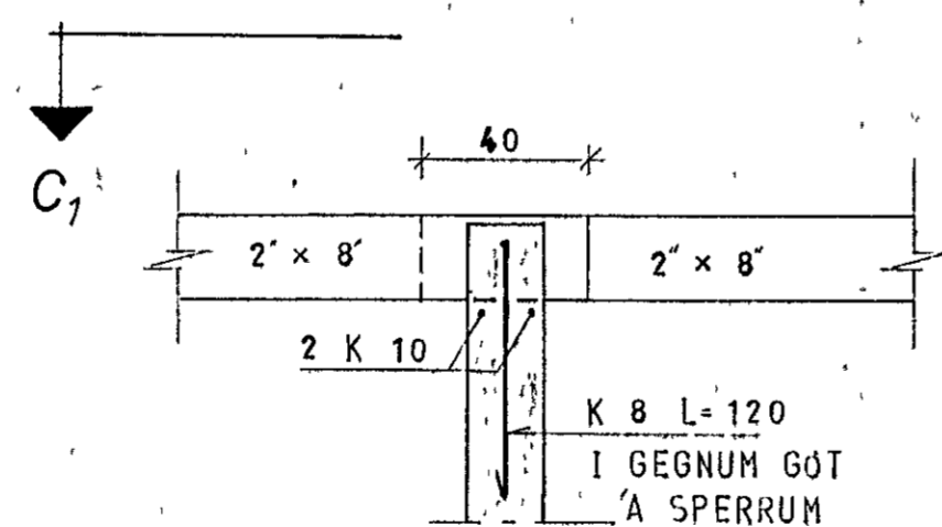
SNID C 1:20
