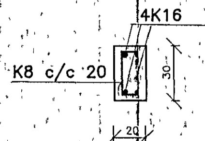
SNID E-E 1:20
