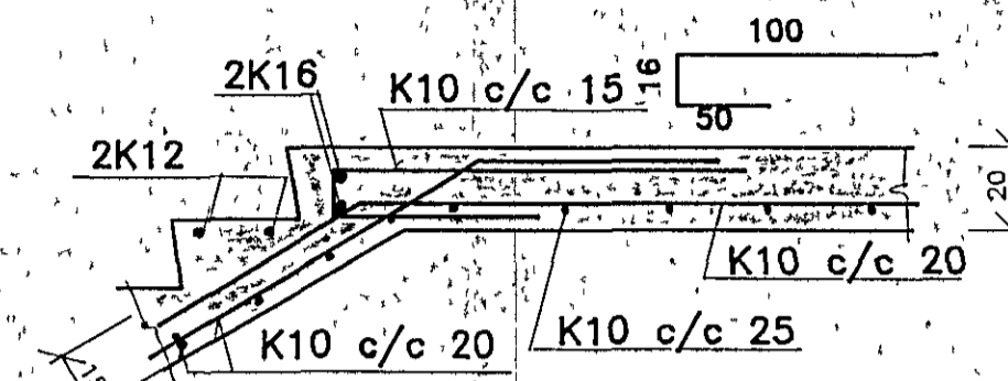
SNID C-C 1:20
