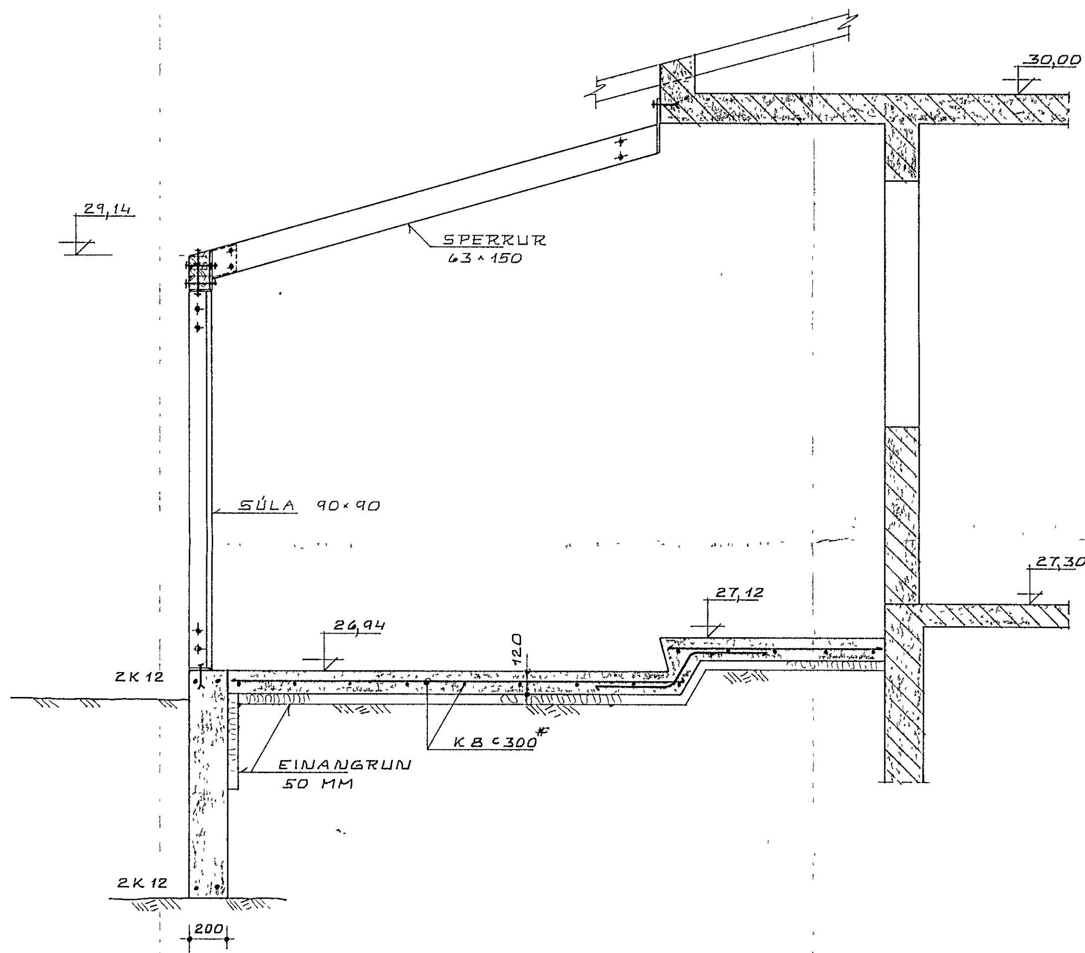
SNID 1 1:20
