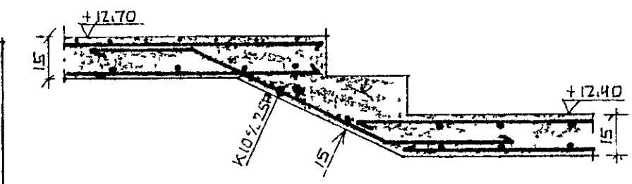
SNID C-C 1:20
