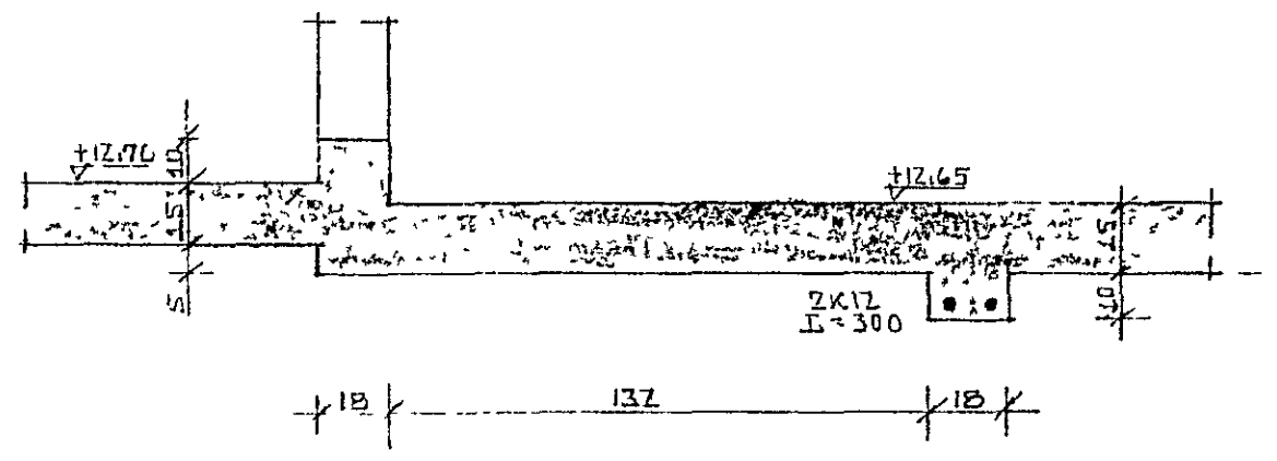
SNID C-C 1:20
