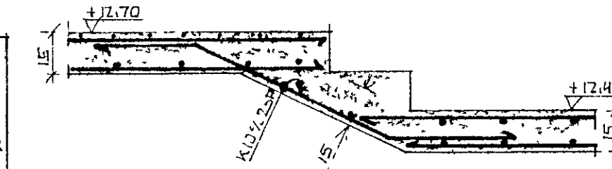
SNID C-C 1:20
