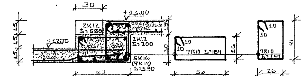
SNID E-E 1:20
