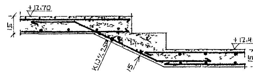
SNID C-C 1:20
