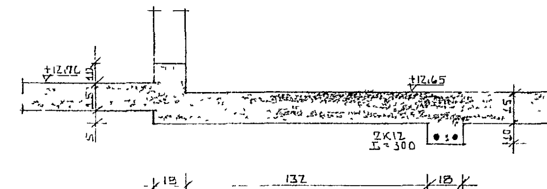
SNID F-F 1:20
