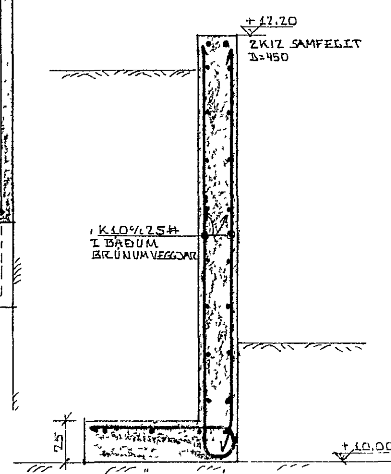
SNID D-D 1:50 SNID E-E
