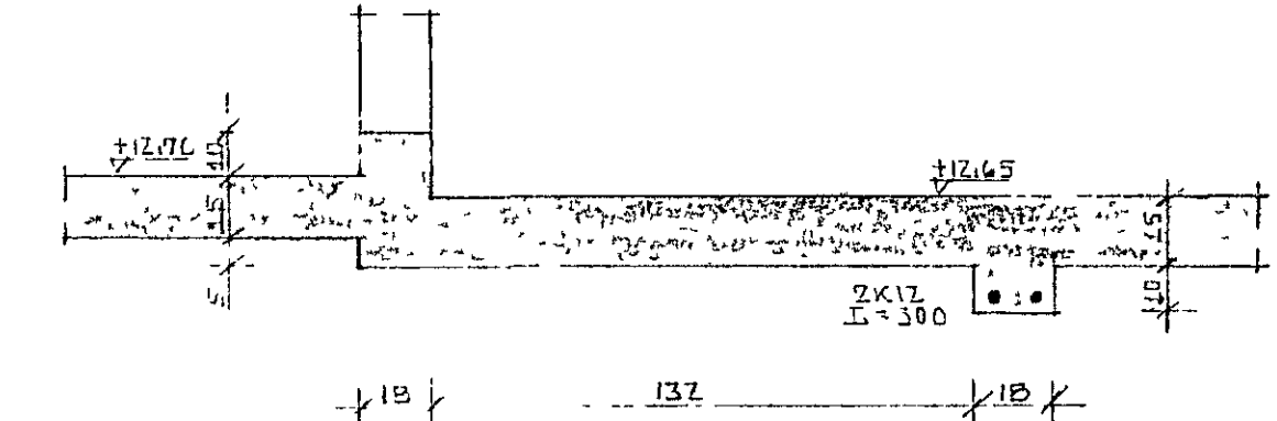
SNID F-F 1:20
