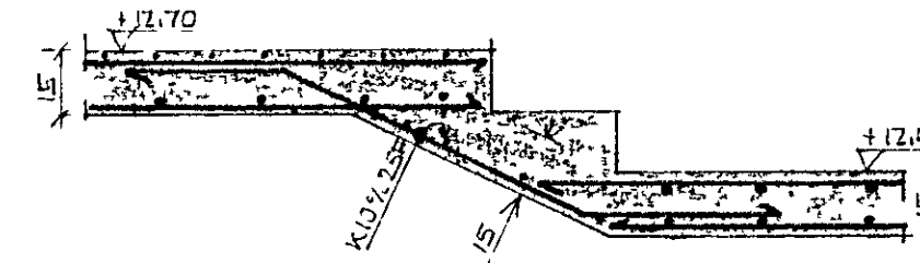
SNID C-C 1:20
