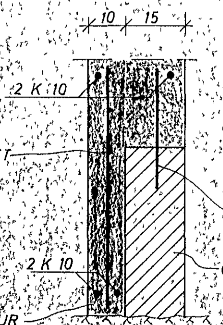
SNID C 1:10
