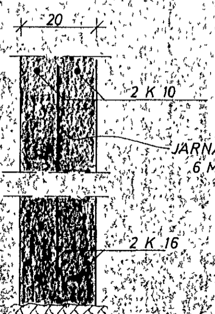
SNID B 1:10
