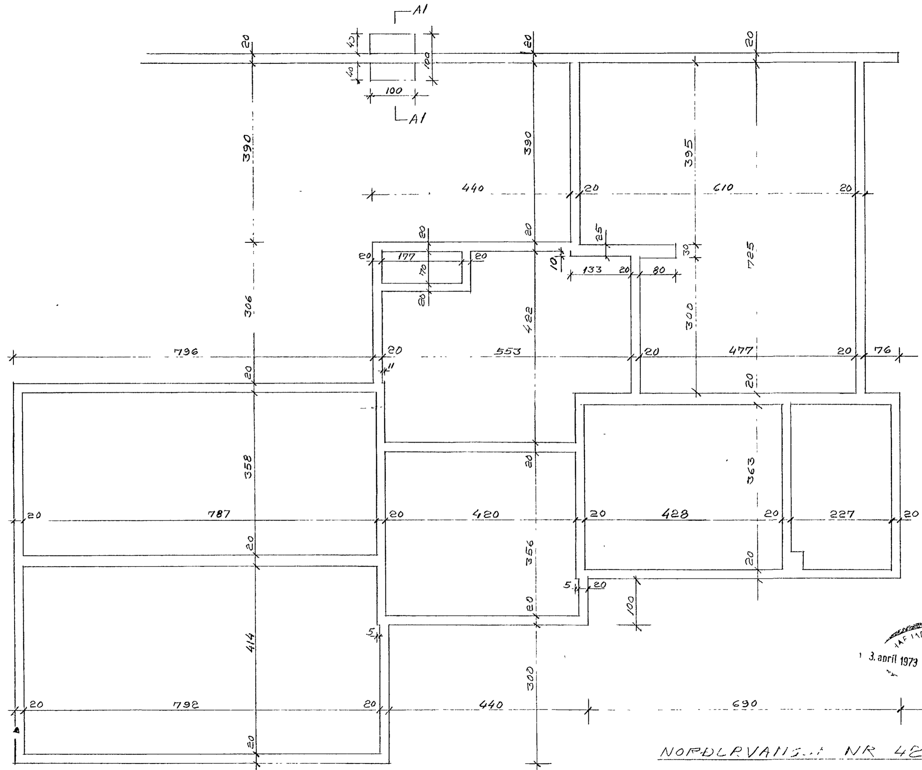
GRUNNPLAN 1:50
