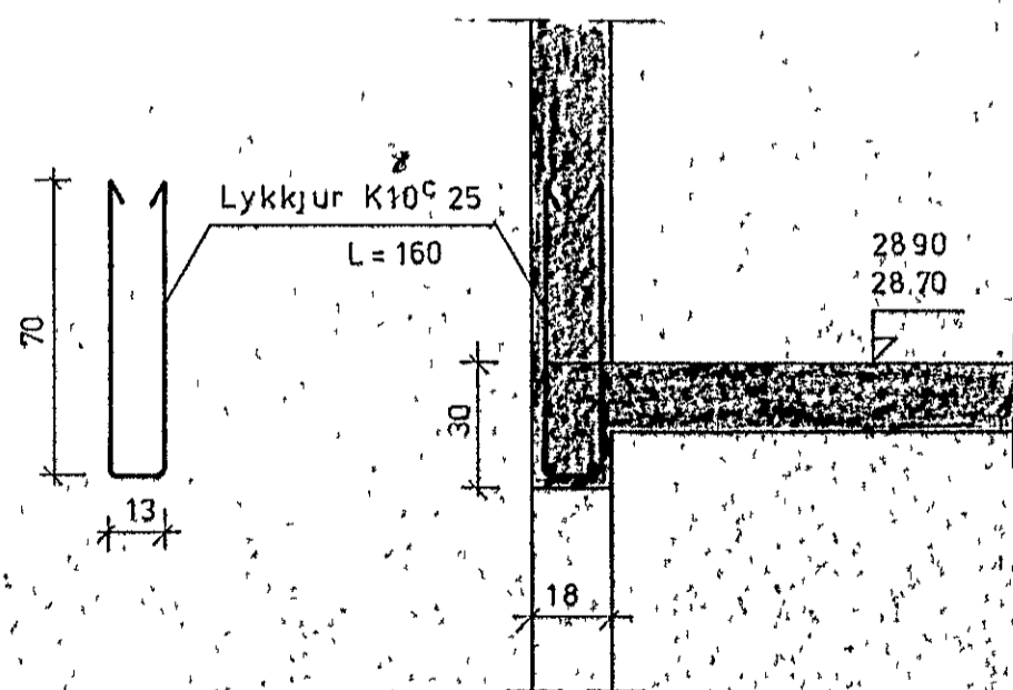
SNID 7-7 1:20
