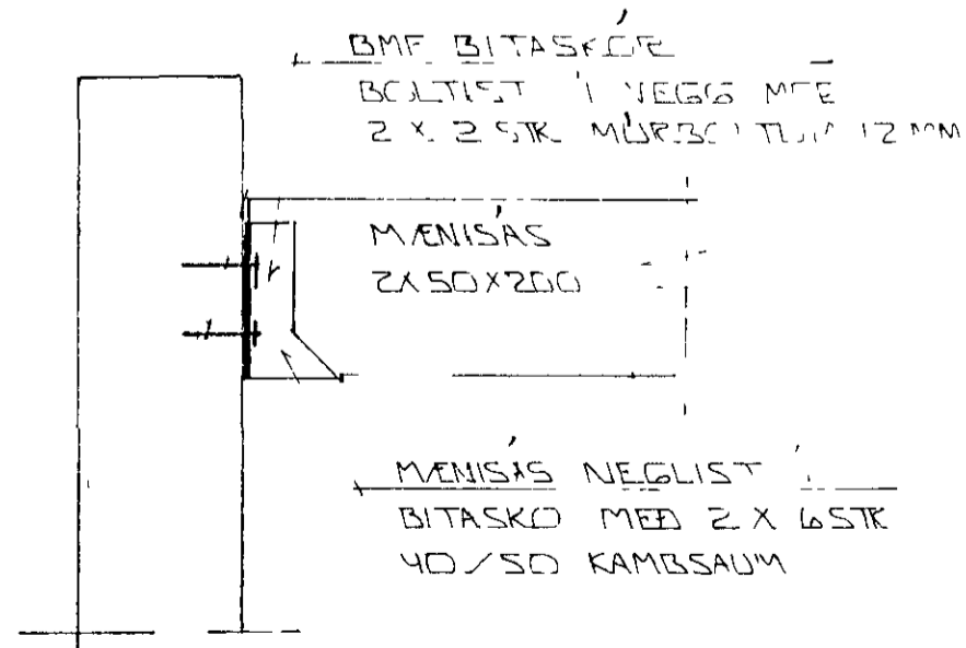
SNIED 3 1:10
