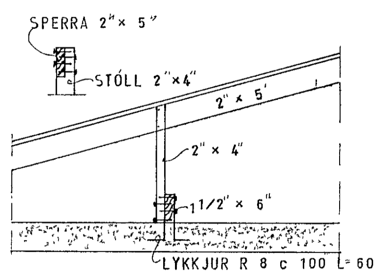
SNID B 1:20
