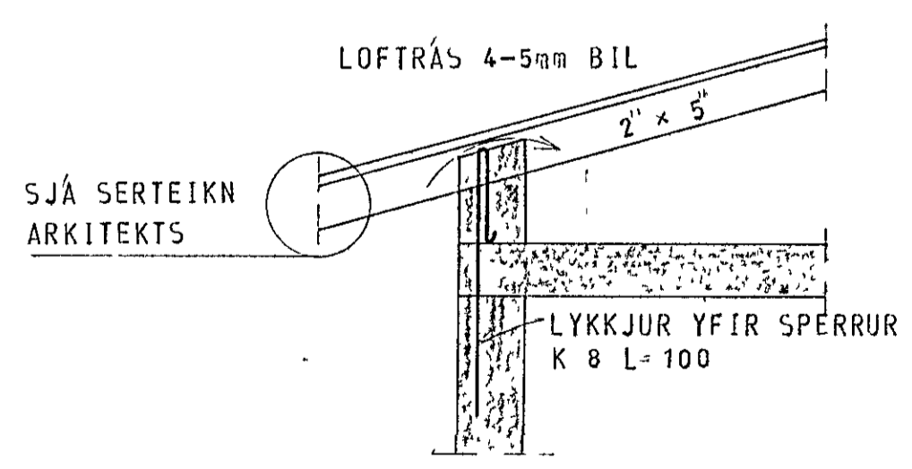
SNID A 1:20
