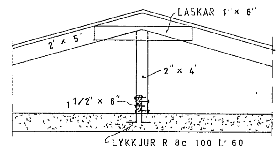
SNID C 1:20
