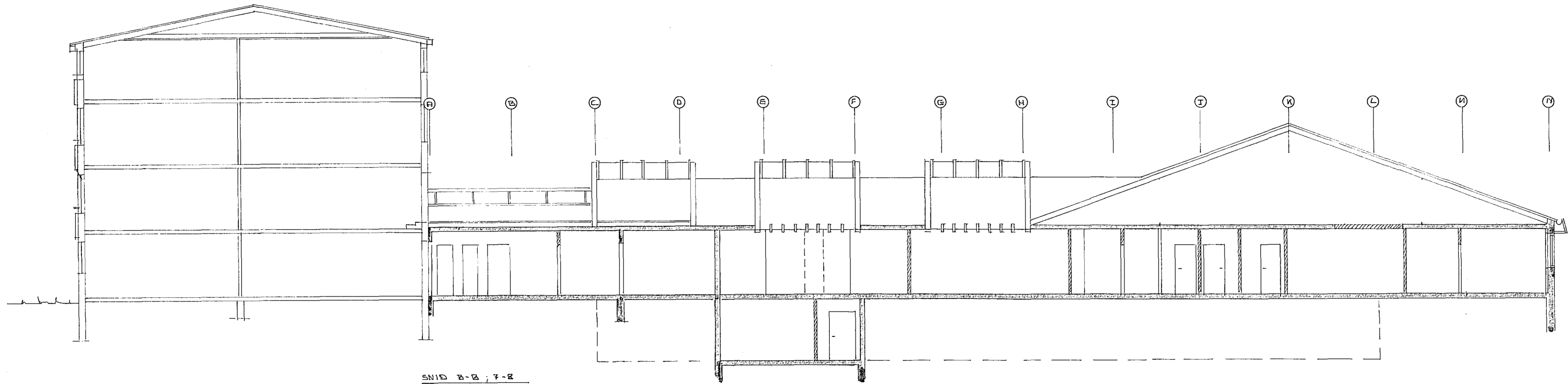
SNID B-B; 7-8
