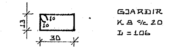
SNID I SULU S2 1:20
