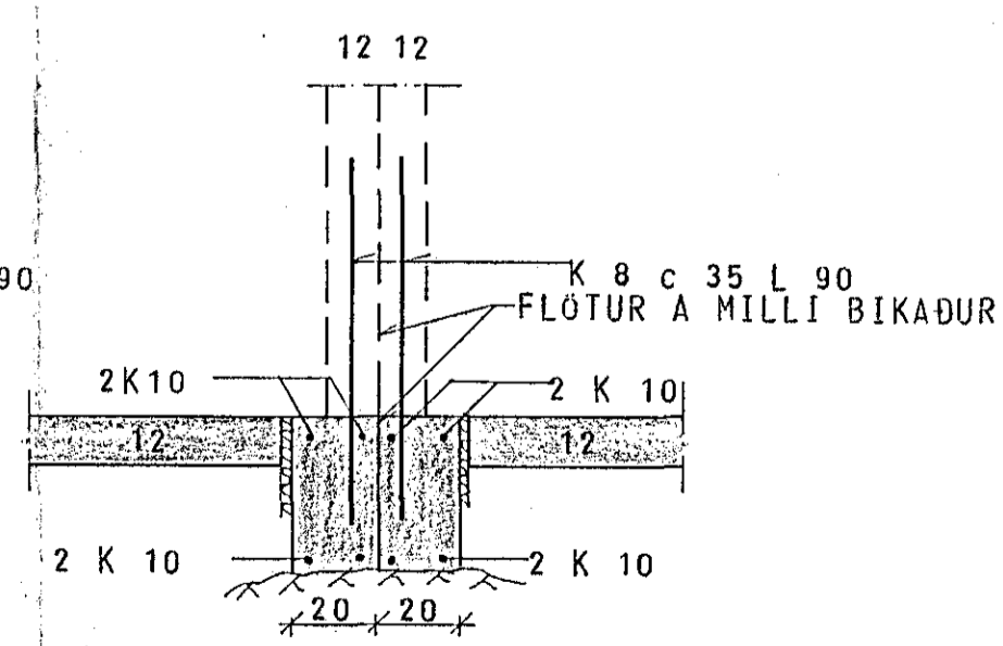
SNID C 1:20
