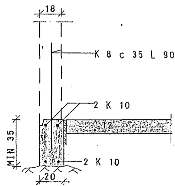
SNID A 1:20
