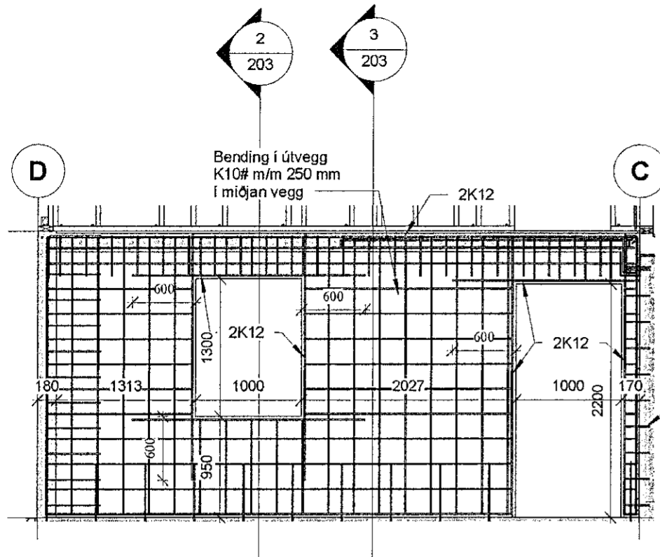
3 Burðarveggur 03 1 : 50
