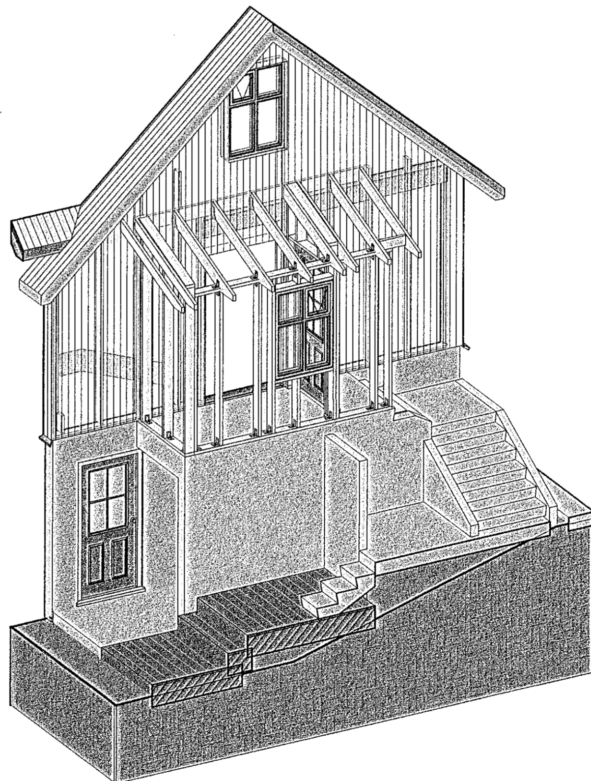
3D burðarvirki - Anddyri
