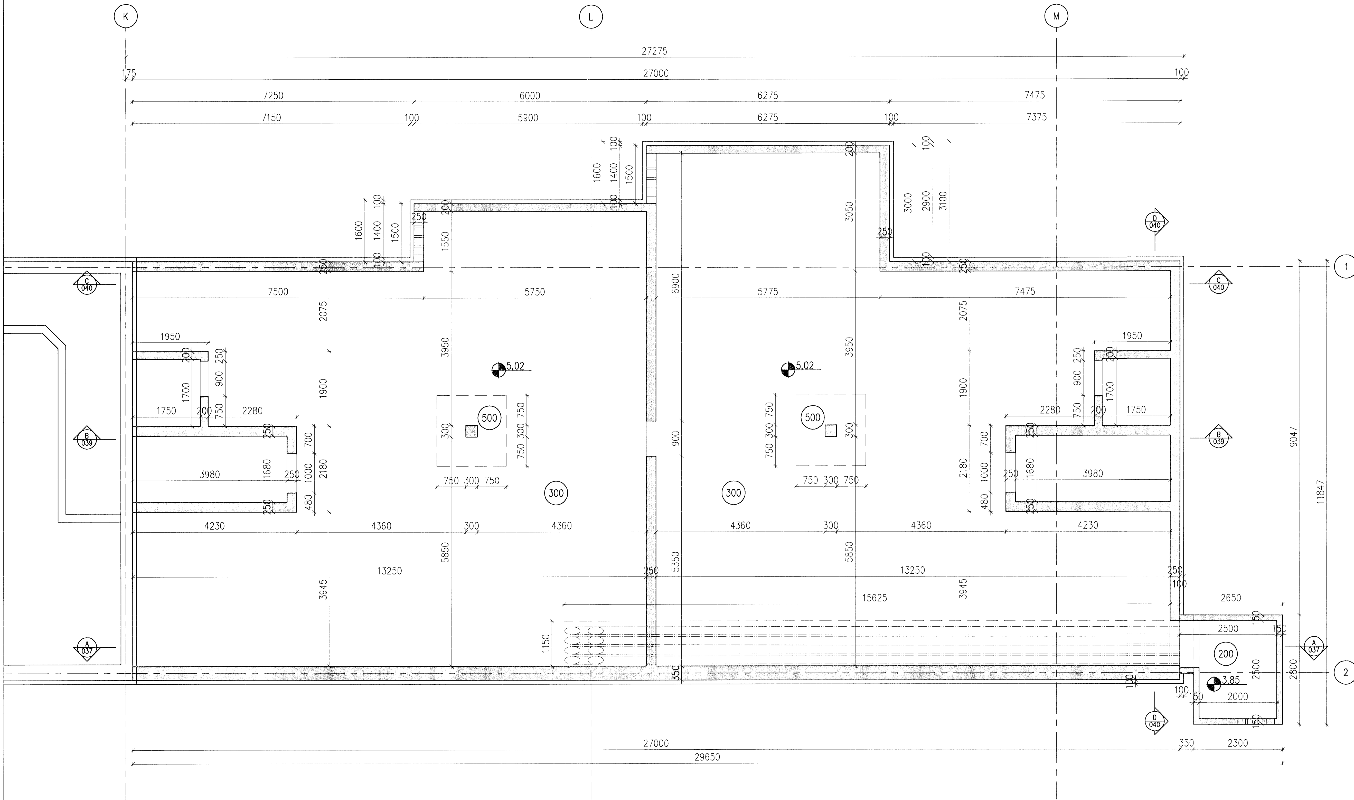
PLAN VIEW, 1:50
