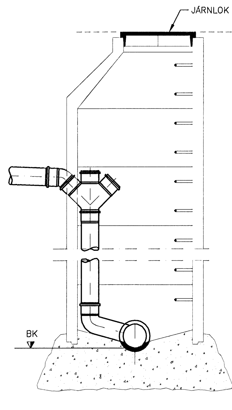
BRUNNUR ø1000
