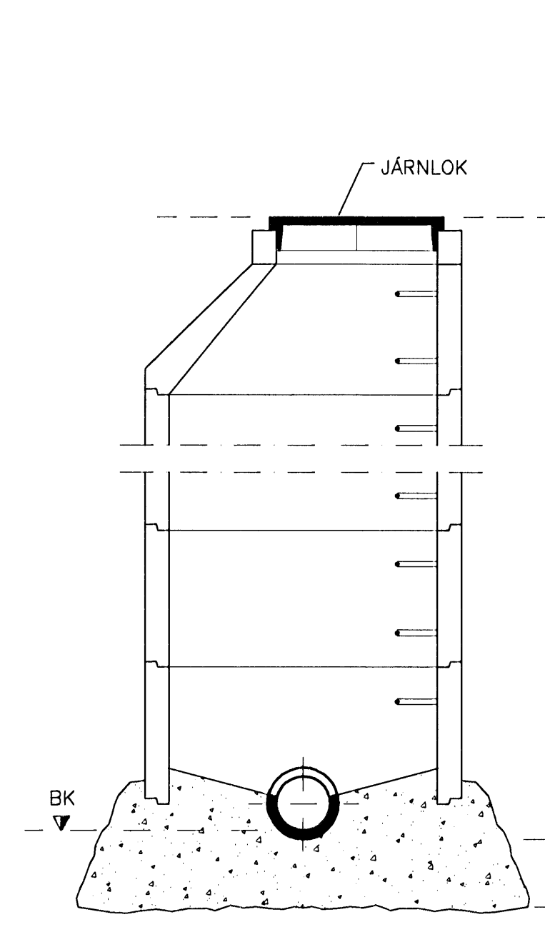
BRUNNUR ø1000
