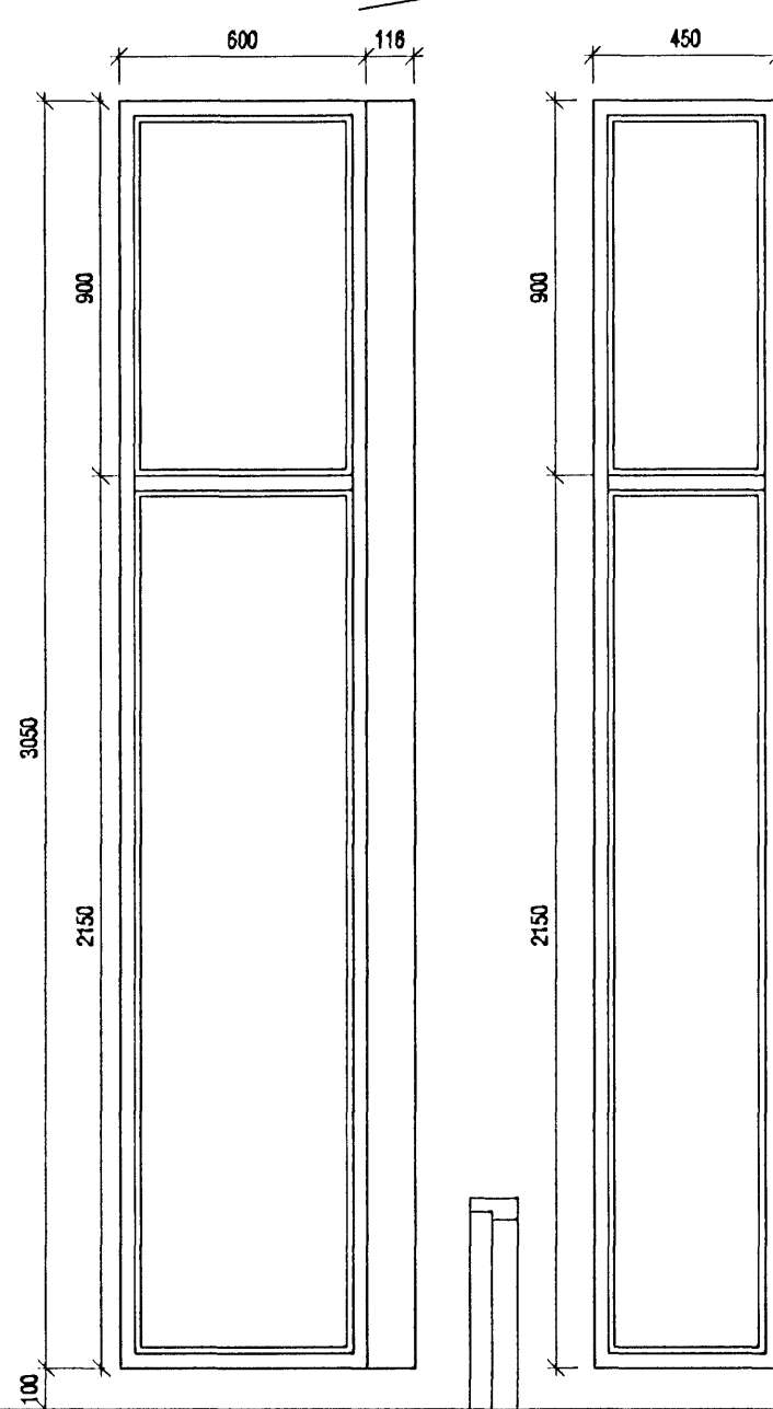
G-2 1 stk.horngluggi
