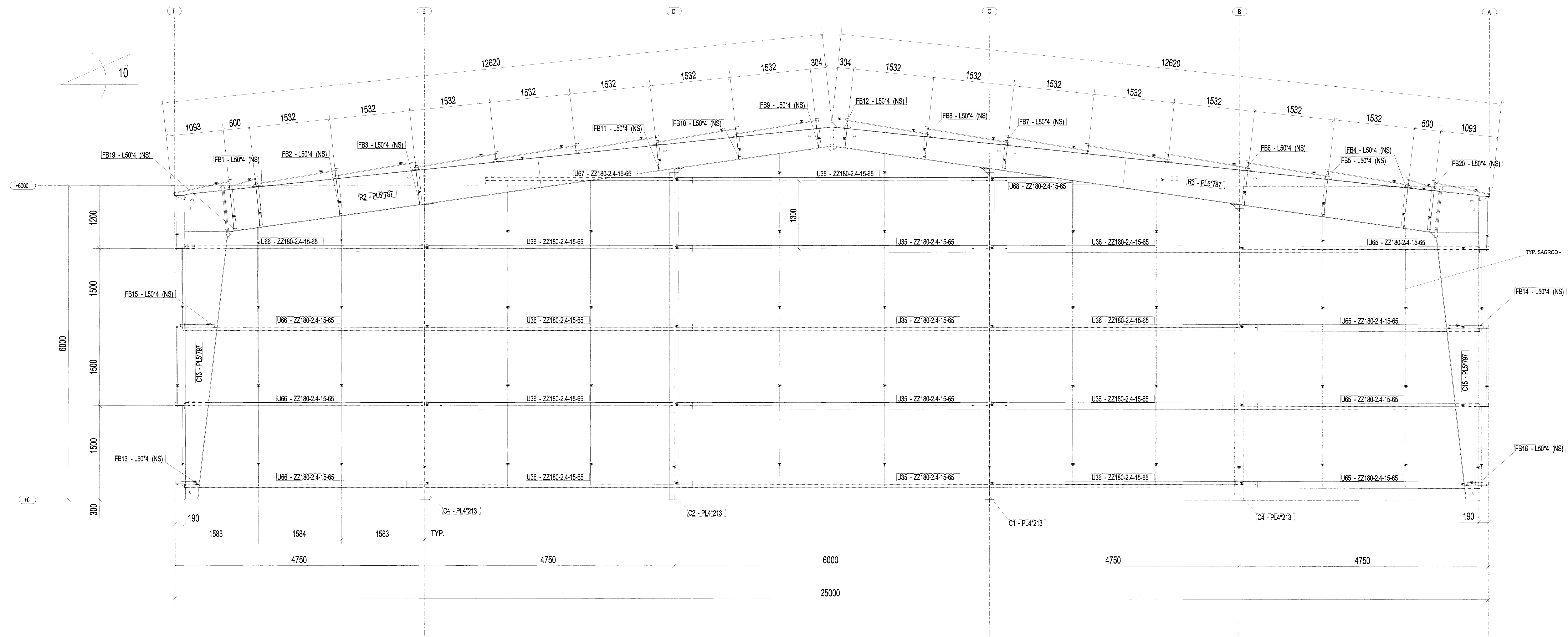
BACK ELEVATION @ GRID 7
