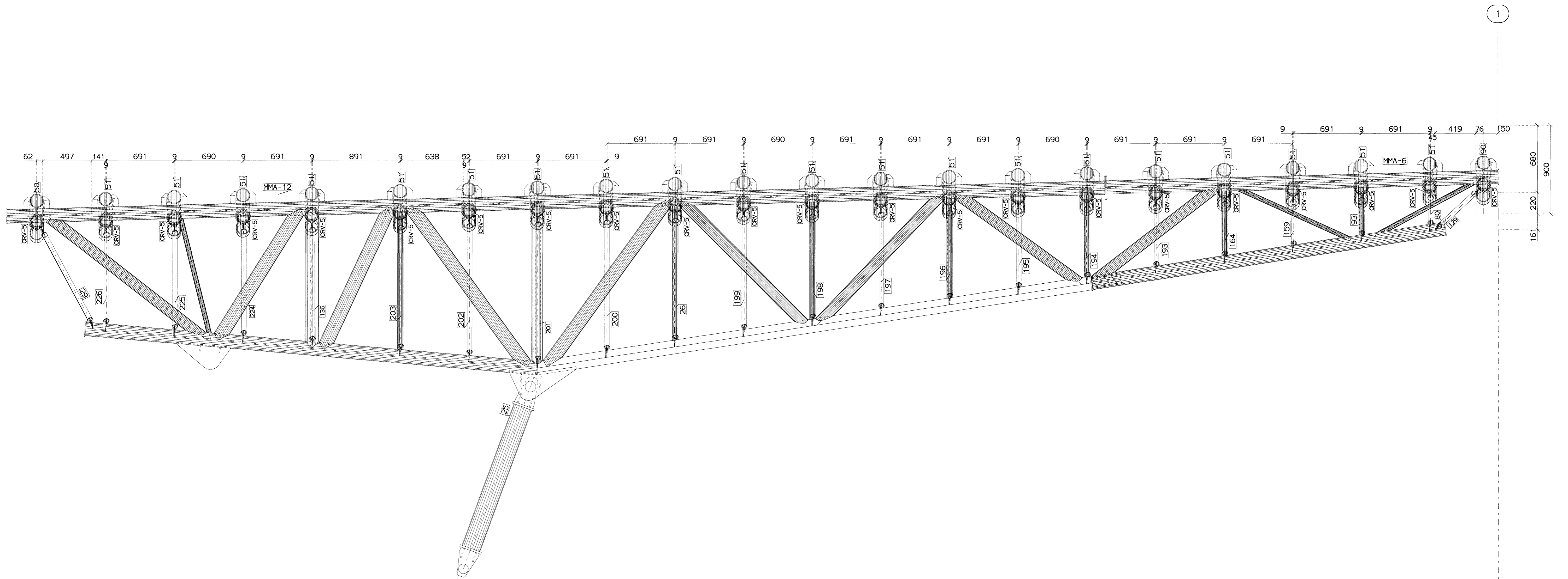
Section
