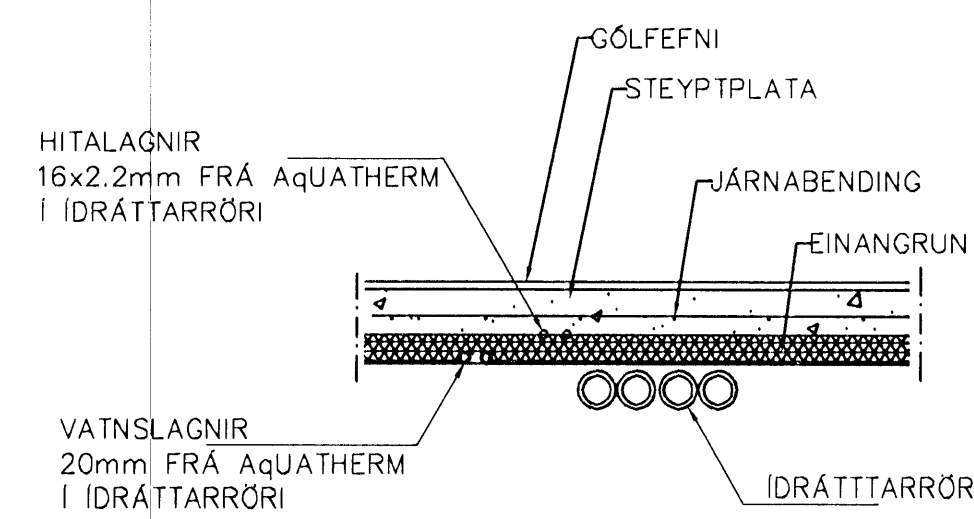
LAGNIR, SNID, 1:20
