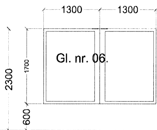
8 STK. HORNGLUGGAR STOFA..
