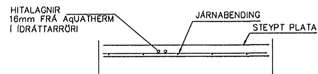
LAGNIR, SNID, 1:20
