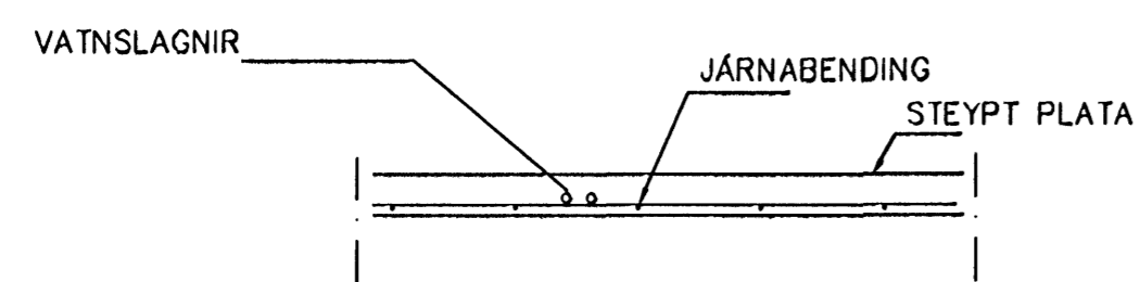
LAGNIR, SNID, 1:20
