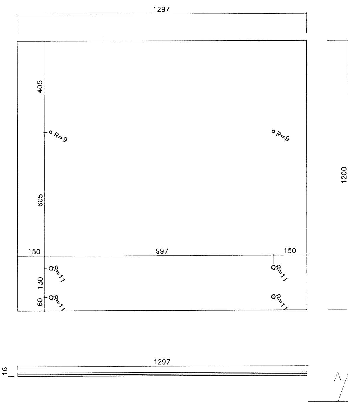
SHG-4, 1297x1200 mm 64 stk.
