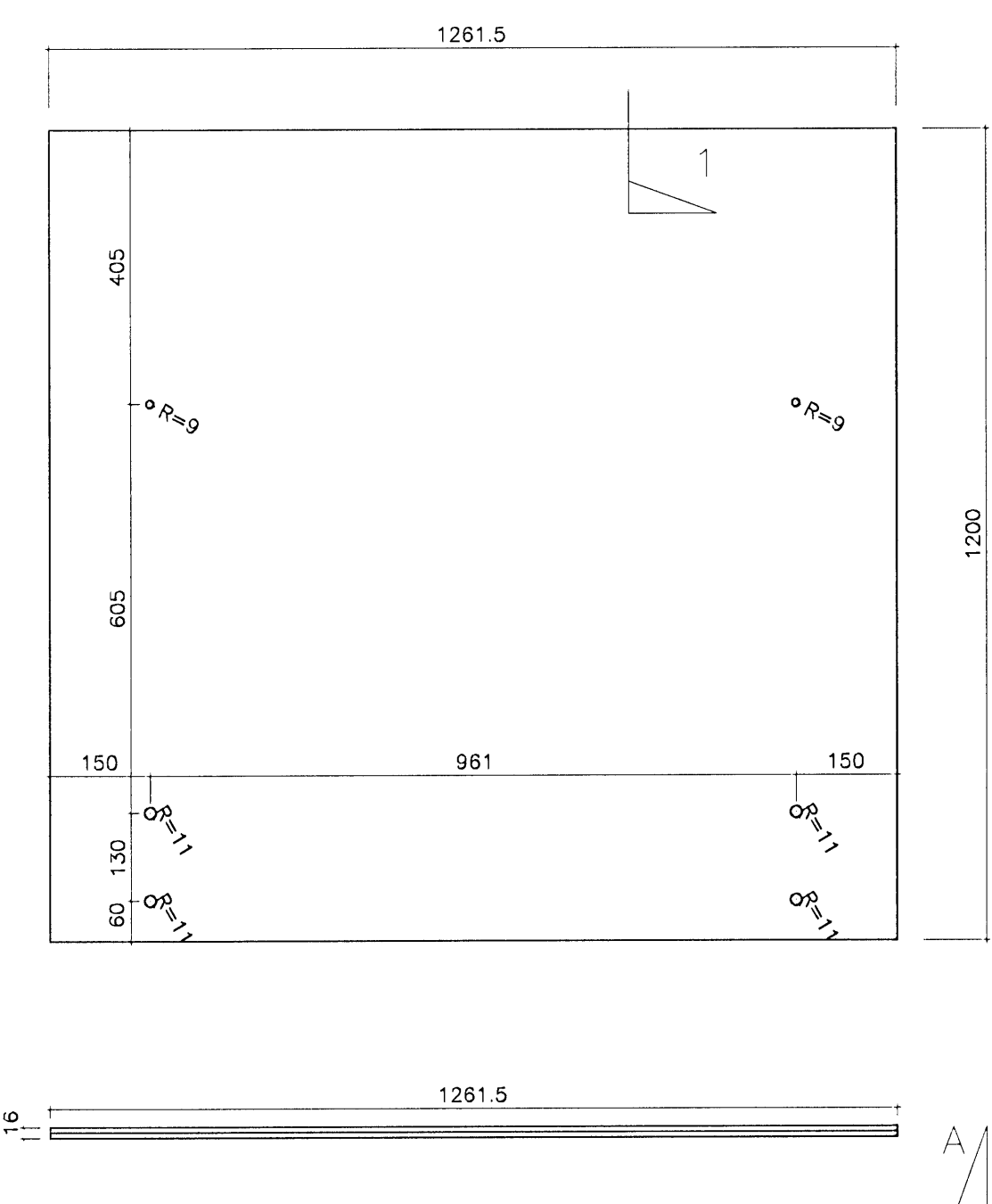
SHG-1, 1261.5x1200 mm 8 stk.
