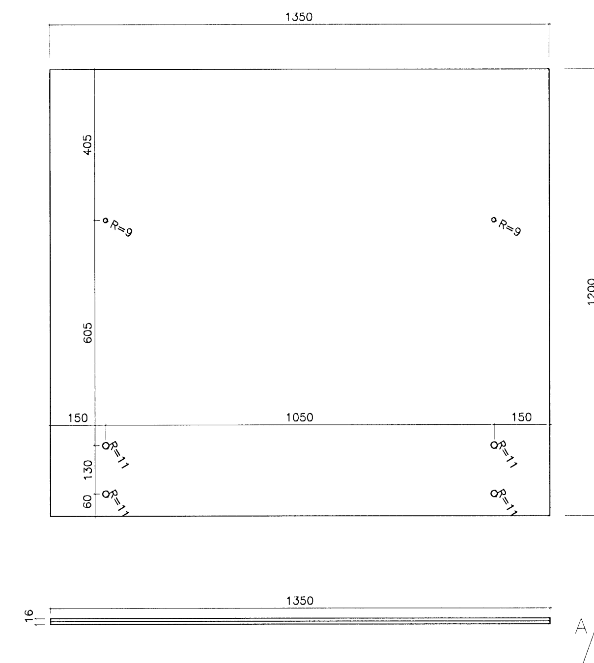
SHG-2, 1350x1200 mm 16 stk.
