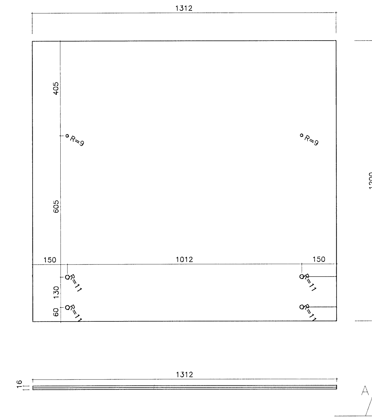
SHG-5, 1312x1200 mm 1 stk.
