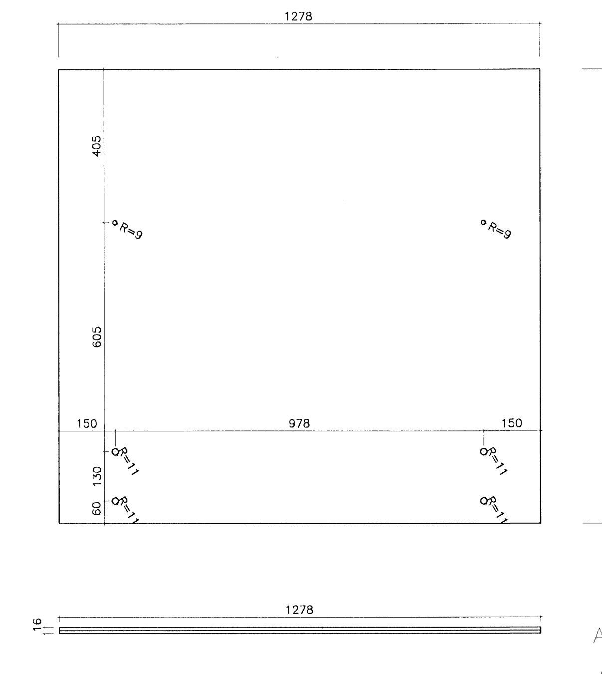
SHG-3, 1278x1200 mm 1 stk.
