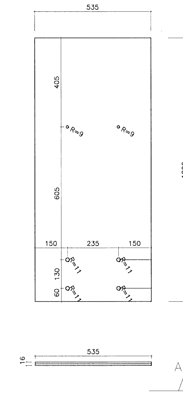
SHG-6, 535x1200 mm 2 stk.
