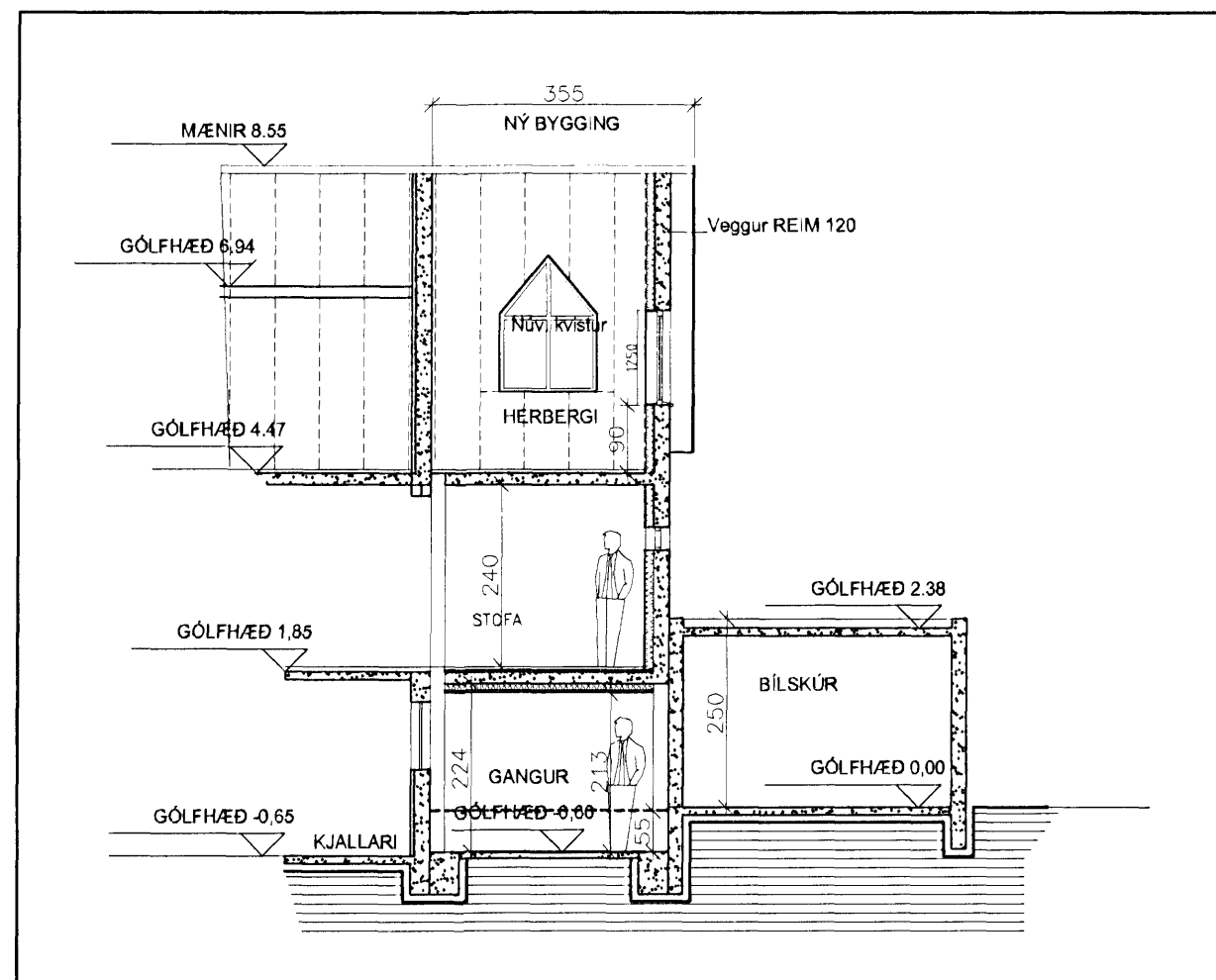
SNID B-B
