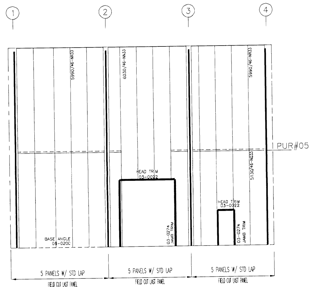
SIDEWALL LINER SHEETING LAYOUT @ GRID - Q Panel = TYPE-R, Base Metal = STEEL, Thickness = 0.50mm., Color = FROST WHITE (AREA#02)
