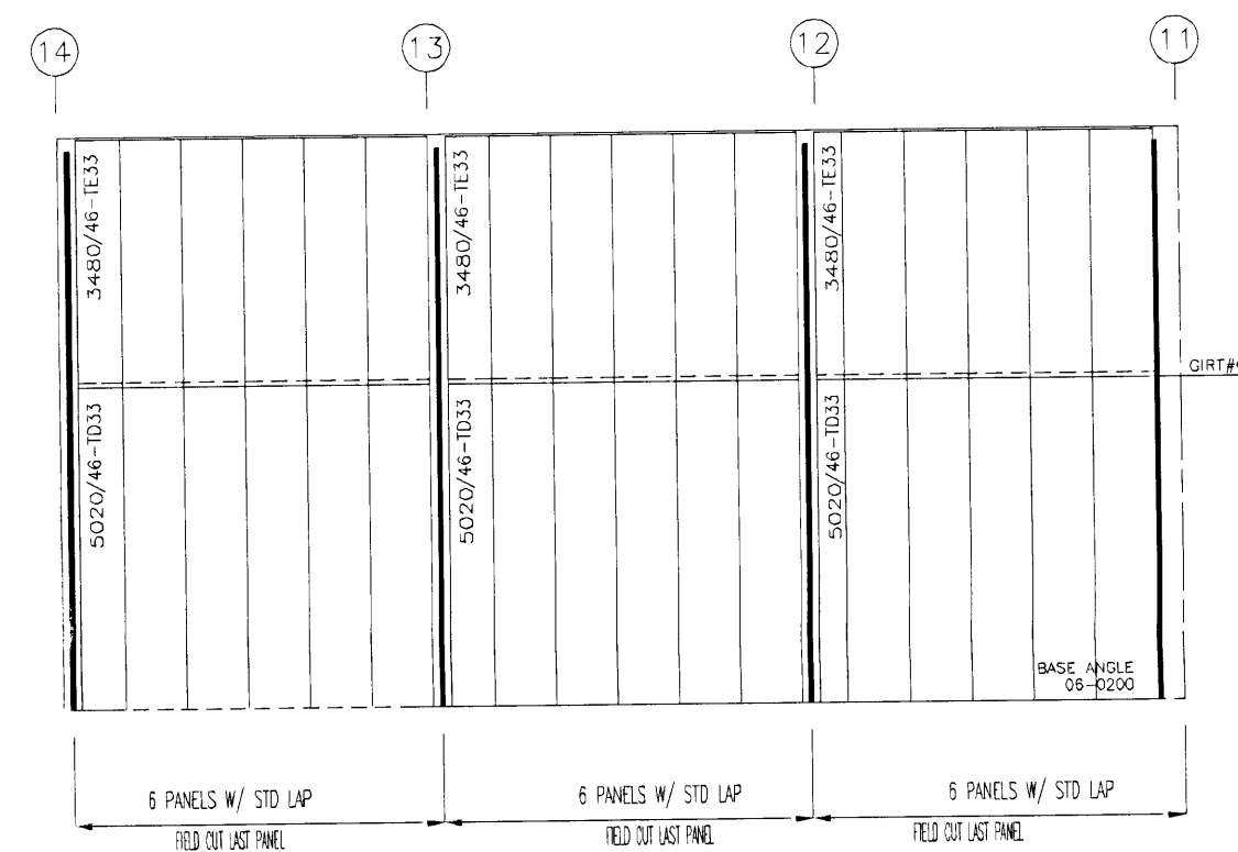
SIDEWALL LINER SHEETING LAYOUT @ GRID - Q Panel = TYPE-R, Base Metal = STEEL, Thickness = 0.50mm., Color = FROST WHITE (AREA#03)
