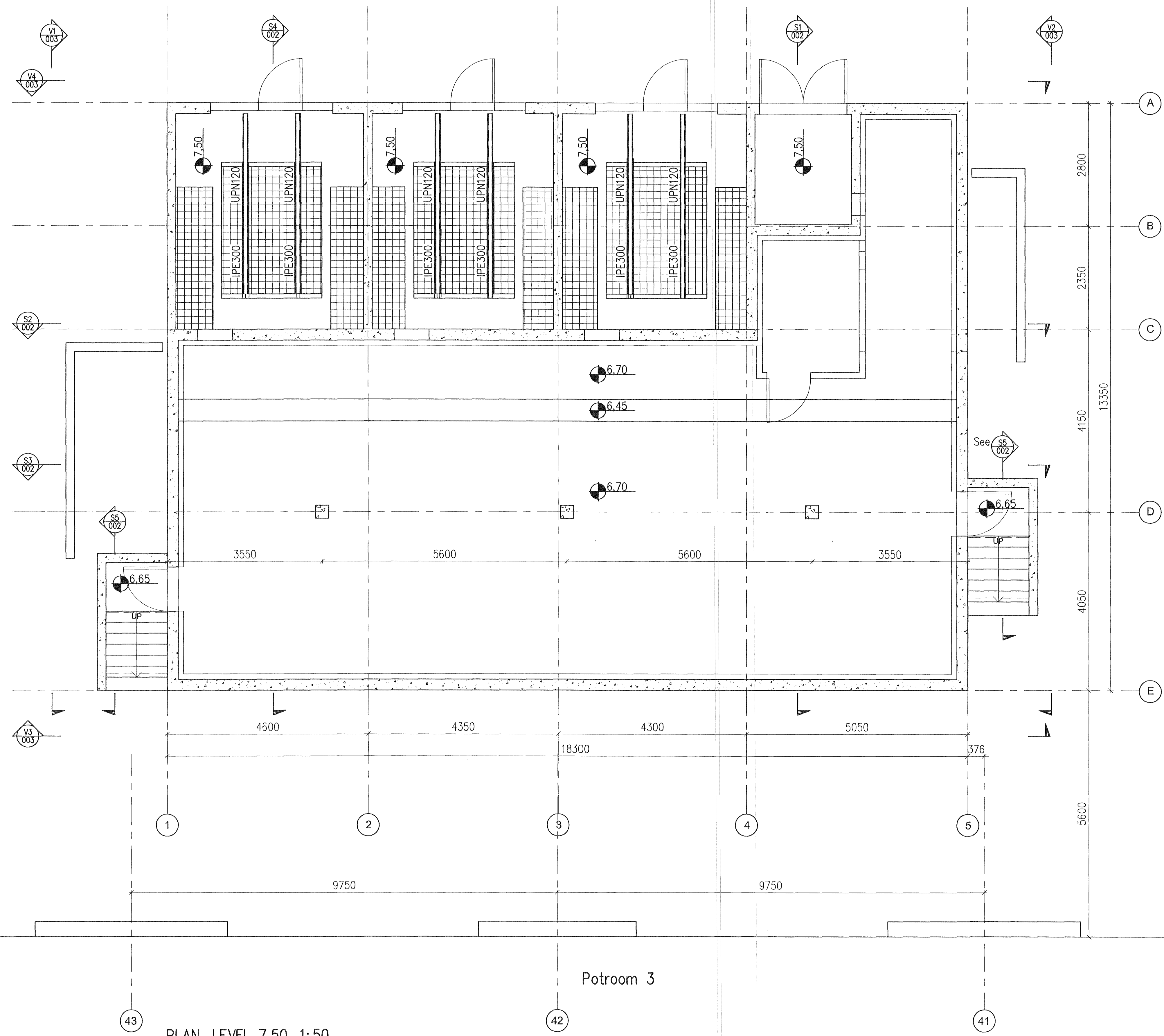
PLAN, LEVEL 7.50, 1:50
