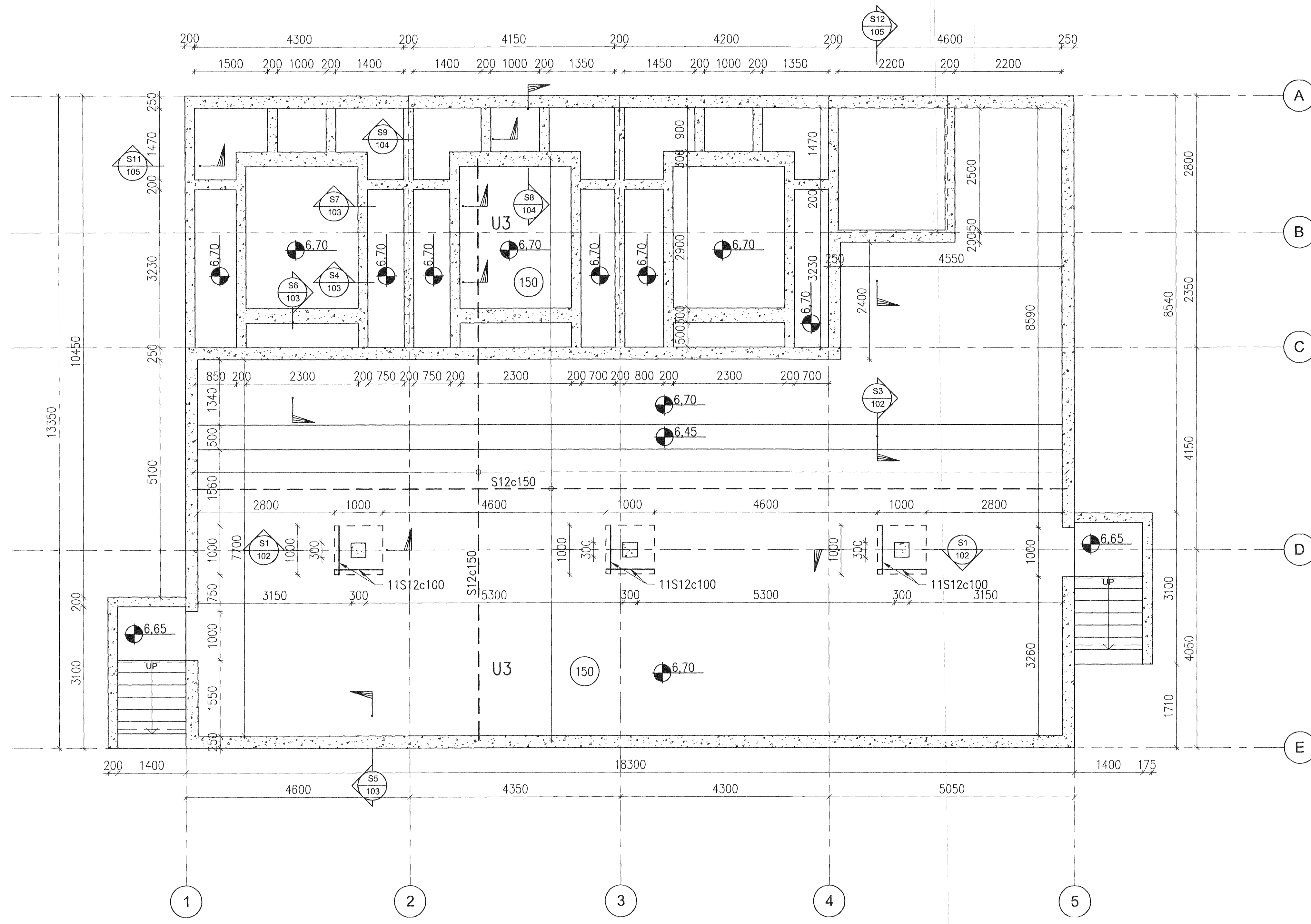
PLAN, LEVEL 6.70, 1:50
