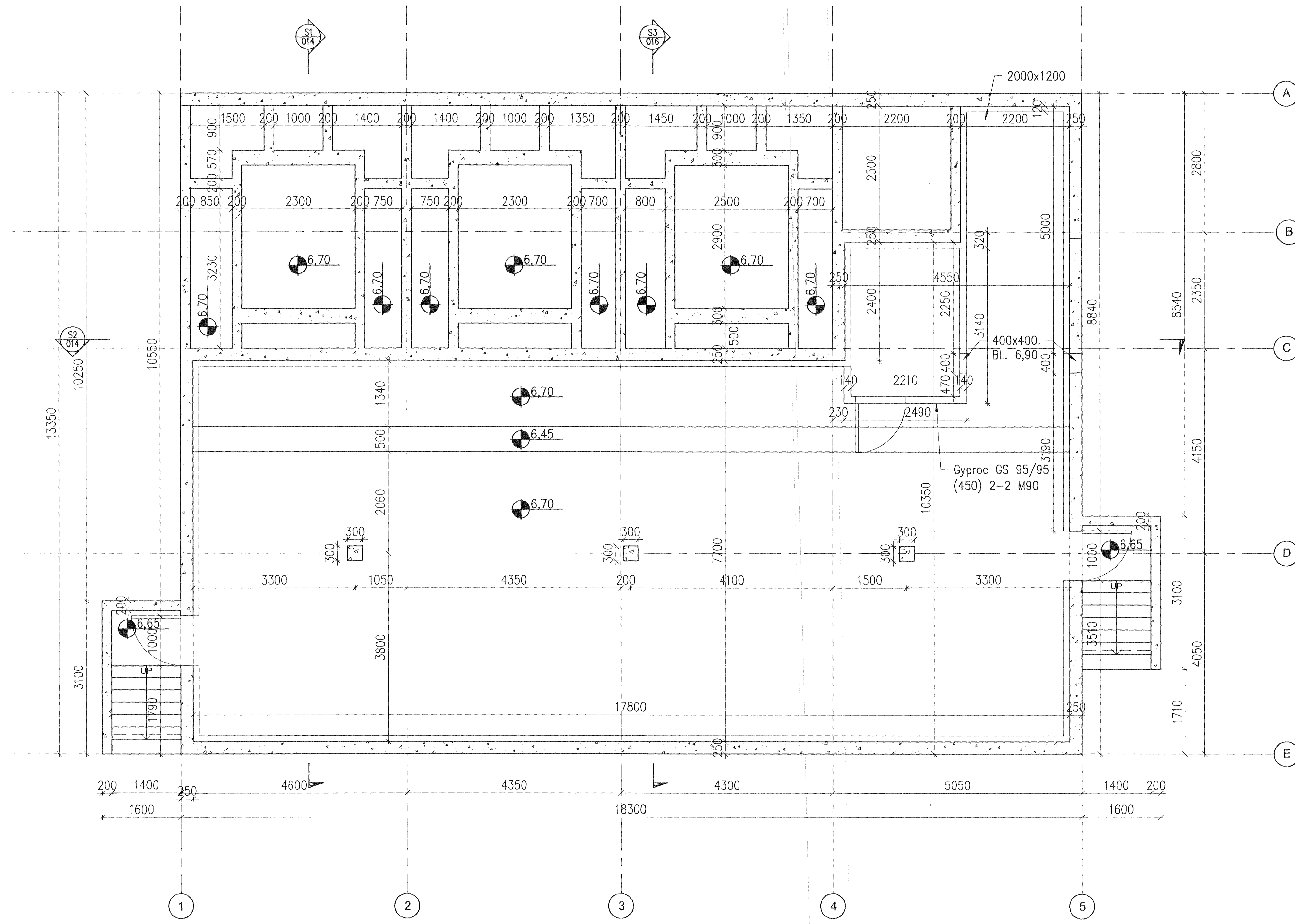
PLAN, LEVEL 6.70, 1:50
