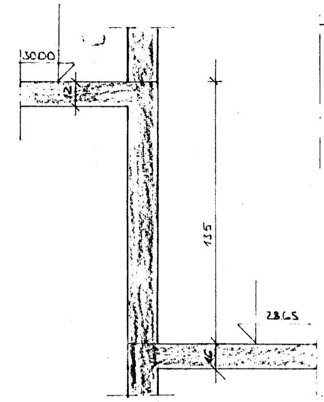
SNID A - A ~ 1:20
