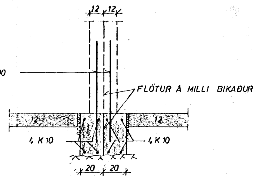
SNID C 1:20
