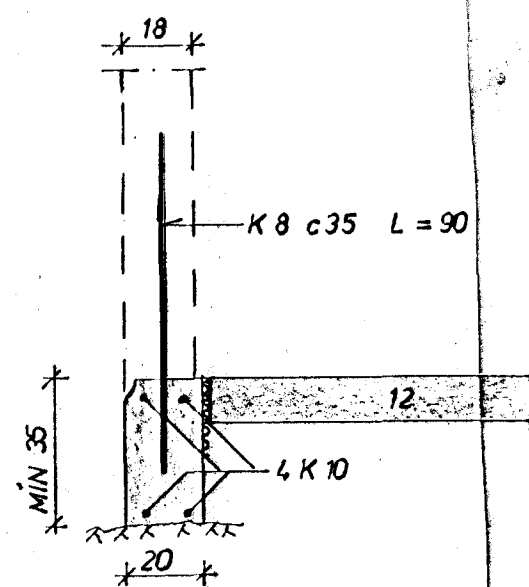
SNID A 1:20
