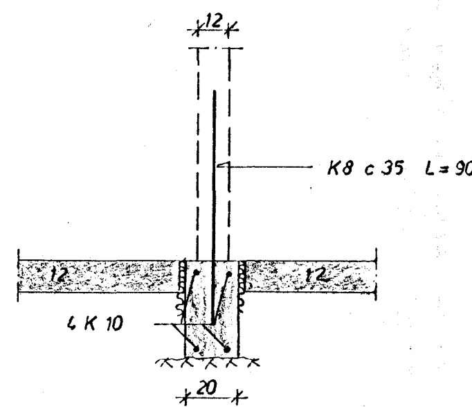
SNID B 1:20
