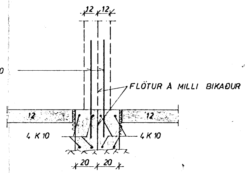
SNID C 1:20
