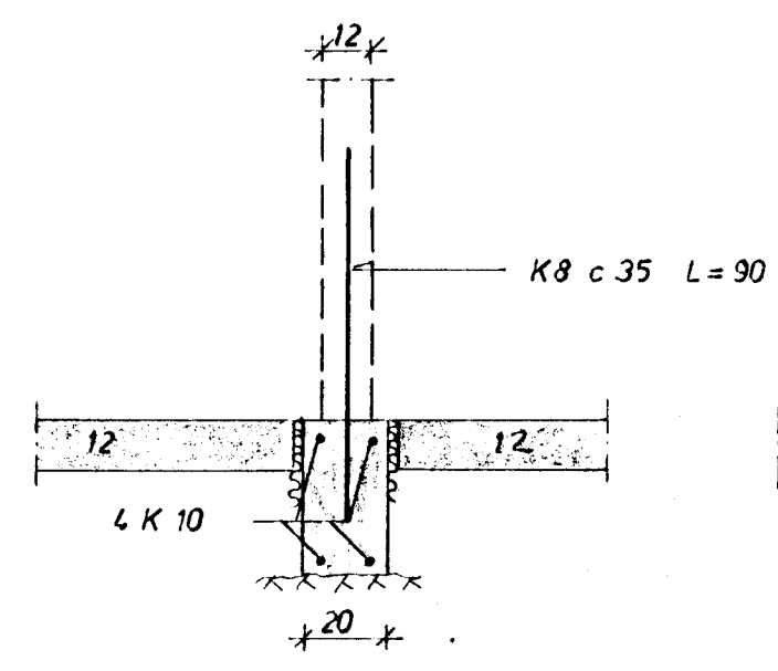
SNID B 1:20
