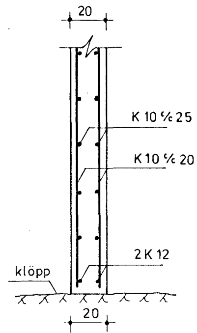
SNID 2-2 mkv. 1:20
