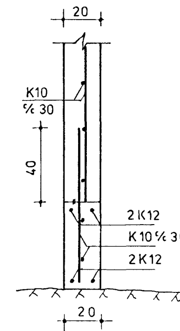
SNID 4-4 mkv. 1:20
