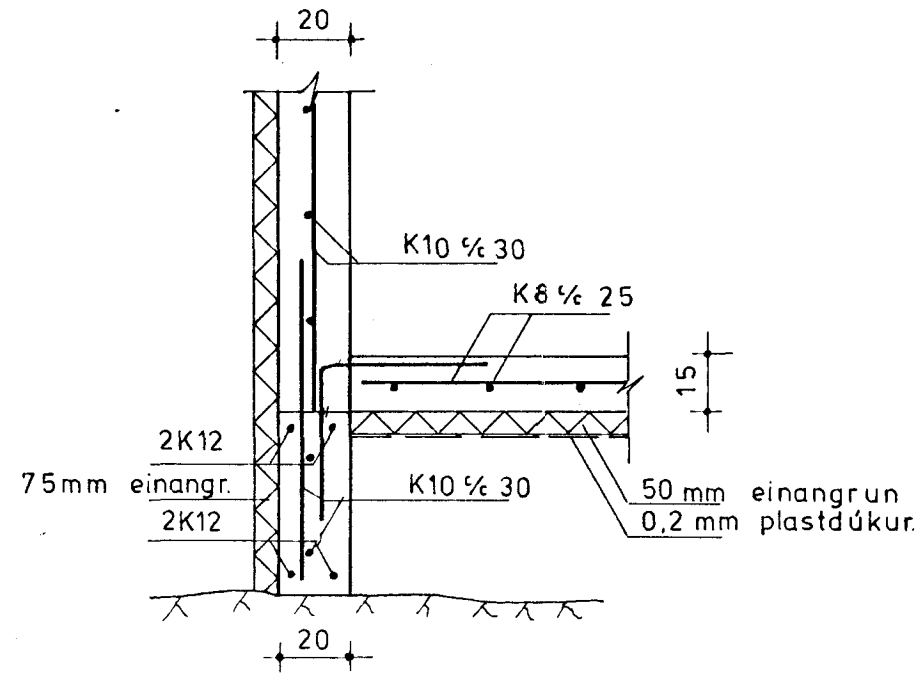
SNID 3-3 mkv. 1:20
